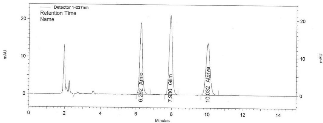
Figure 3.15. Chromatogram of amlodipine, glimepiride, and atorvastatin using 234 nm wavelength.
